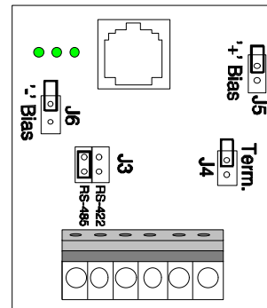
RS-485 Jumper locations for units on intermediate drops of the network.
